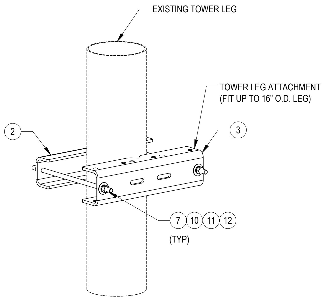
ROUND TOWER LEG ATTACHMENT DETAIL
