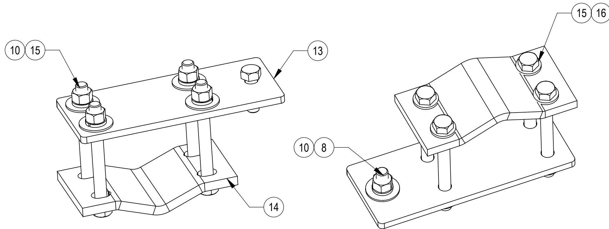
ADAPTER FOR PIPE CONNECTION
