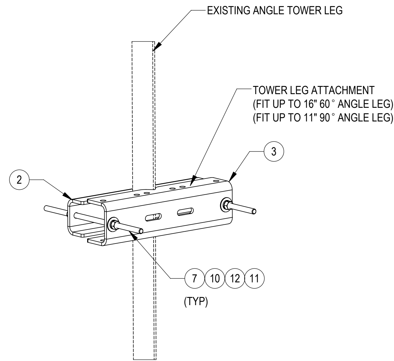
ANGLE TOWER LEG ATTACHMENT DETAIL
