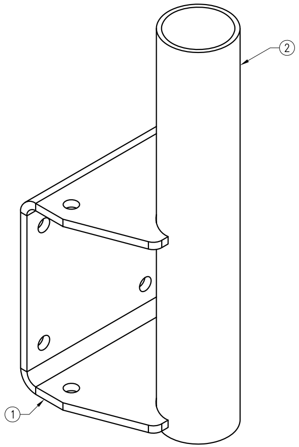
COLLAR MOUNT STANDOFF ADAPTER ISOMETRIC VIEW
