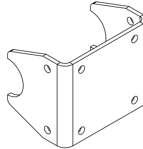
P574-020-01 ISOMETRIC VIEW
