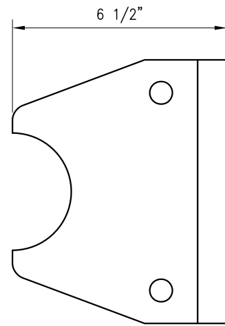
AFTER BENDING SIDE VIEW
