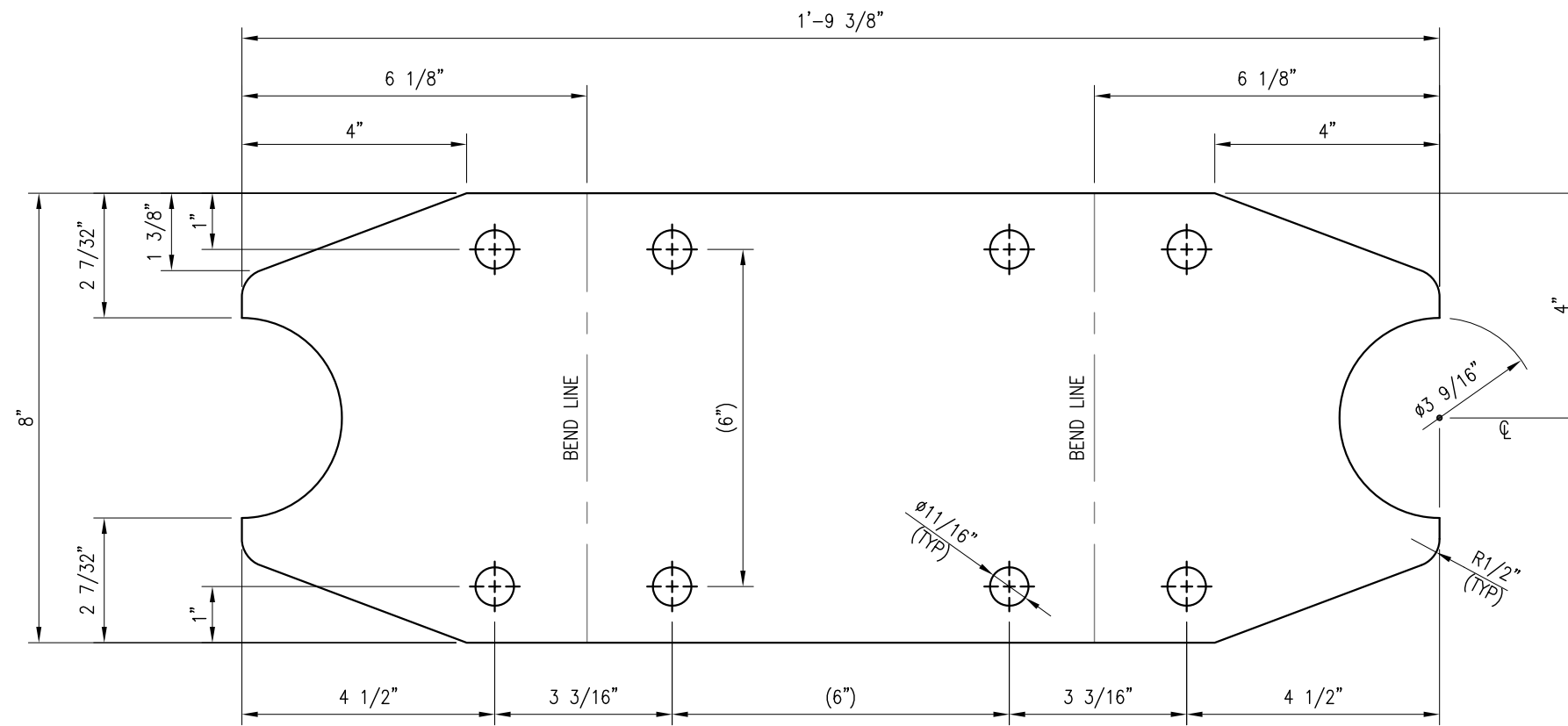
BEFORE BENDING P574-020-01 PL 3/8" X 8" X 1'-9 3/8" A36 BENT PLATE (14.39 LBS)
