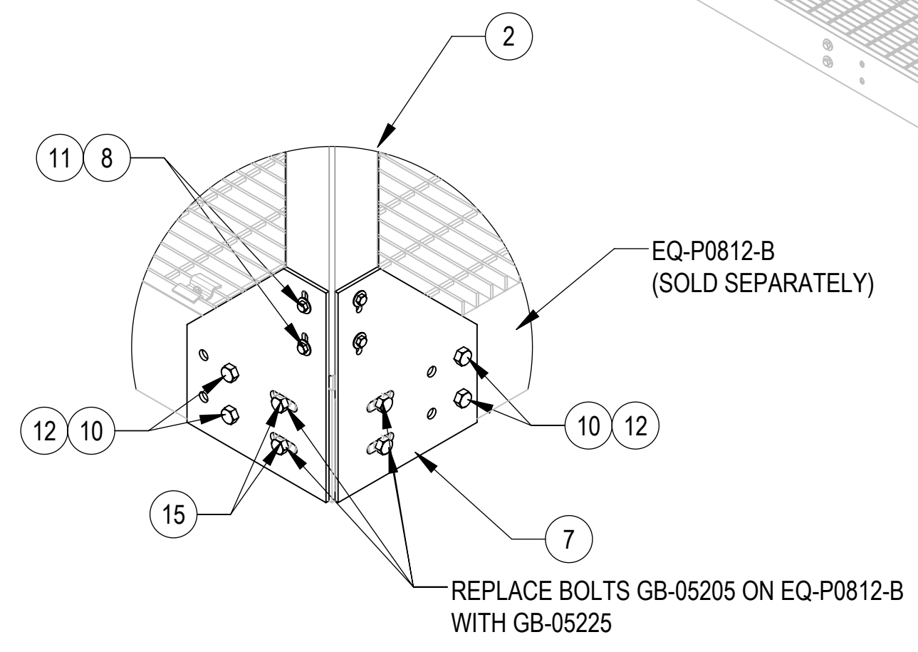
DETAIL D SCALE 1 : 8 (4 PLACES)
