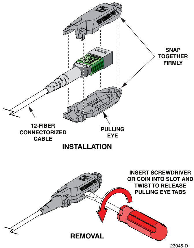
Figure 1. Rapid Fiber Single Cable Pulling Eye Installation and Removal
