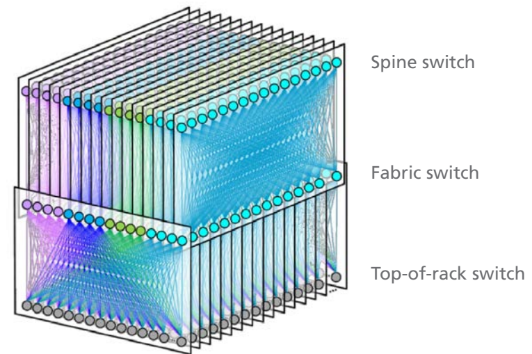
Fig. 2: FaceBook F16 data center network topology (source: https://engineering.fb.com/2019/03/14/data-center-engineering/f16-minipack/ )
