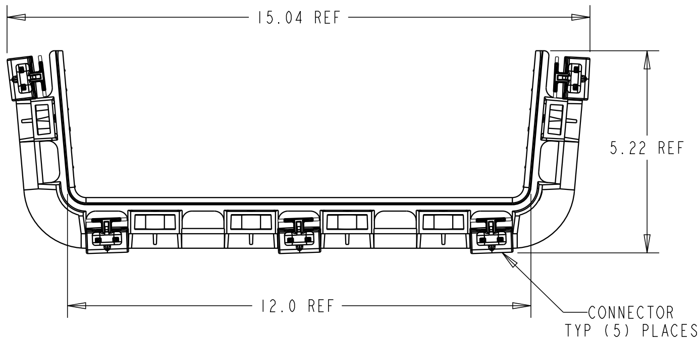
DETAIL C 4 X 12 JUNCTION
