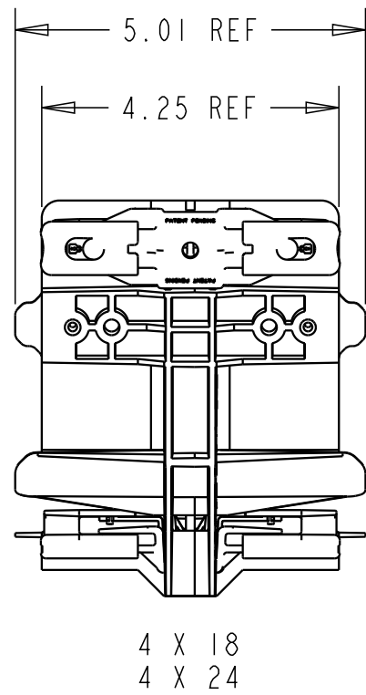
DETAIL D 4 X 18 JUNCTION
