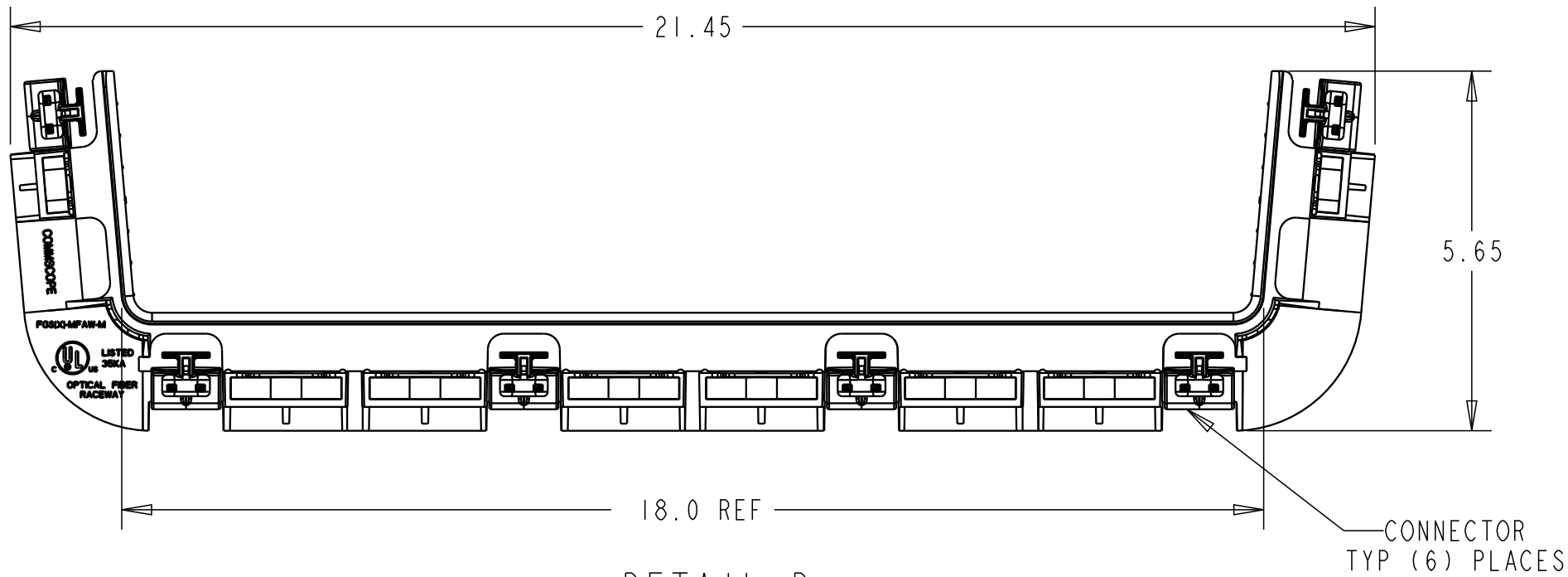
DETAIL D 4 X 18 JUNCTION
