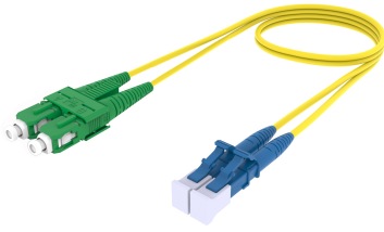
Fiber Optic Patch Cord, Duplex, Singlemode, LC/UPC to SC/APC 9°, yellow, 1 m
