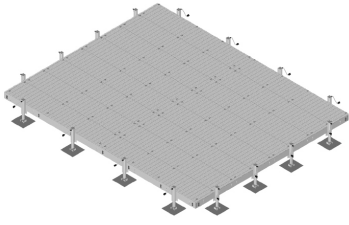
Equipment Platform, 20 ft x 20 ft, base with sixteen adjustable legs
