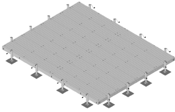
Equipment Platform, 18 ft x 20 ft, base with sixteen adjustable legs
