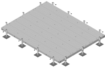
Equipment Platform, 16 ft x 18 ft, base with sixteen adjustable legs
