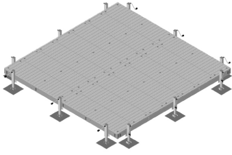
Equipment Platform, 14 ft x 14 ft, base with twelve adjustable legs
