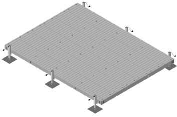
Equipment Platform, 12 ft x 12 ft, base with six adjustable legs
