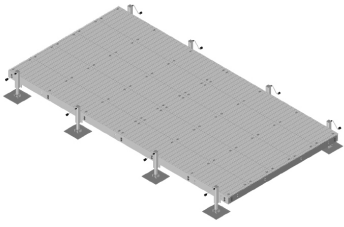
Equipment Platform, 10 ft x 20 ft, base with eight adjustable legs
