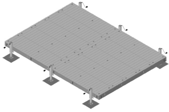
Equipment Platform, 10 ft x 15 ft, base with six adjustable legs
