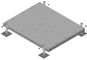
Equipment Platform, 8 ft x 10 ft, base with four adjustable legs
