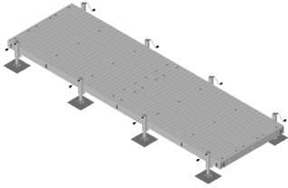
Equipment Platform, 6 ft x 20 ft, base with eight adjustable legs
