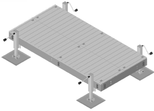
Equipment Platform, 4 ft x 10 ft, base with four adjustable legs
