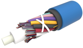
24 Core OM4 50/125µm, Gel-filled Loose Tube Cable, OD 6.3mm
