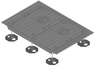
Light Duty Equipment Platform, 4 ft x 6 ft, with six light duty legs
