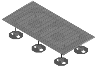
Light Duty Equipment Platform, 3 ft x 6 ft, with six light duty legs
