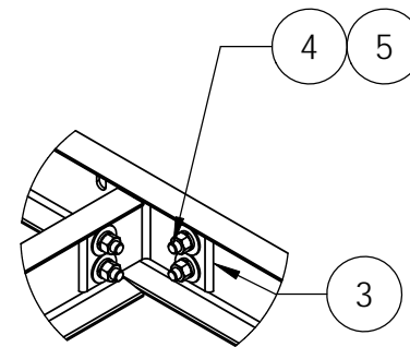
DETAIL A SCALE 1 : 11
