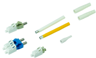
Behind The Wall Pre-Radiused LC APC Connector for 0.9 mm Fiber, single-mode
