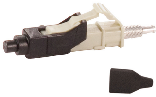
LightCrimp Plus™ Fiber Optic Kit, LC, simplex, 50/125 μm, jacketed
