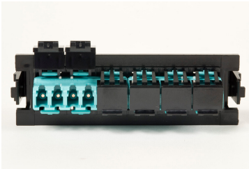
G2 Modular Bezel with 12 LazrSPEED® Multimode LC Adapters, No Pigtails
