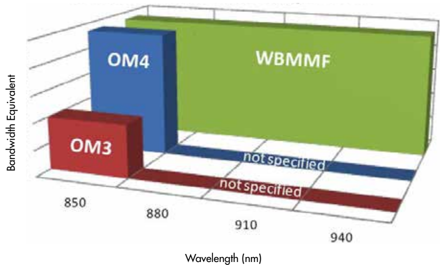
Figure 23. A comparison of total bandwidth between OM3, OM4, and WBMMF
