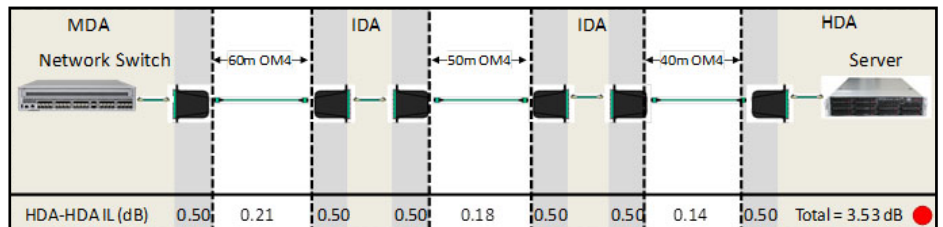
Figure 14. Loss budget calculations for server-to-network link over OM4 fibre - additional connections added
