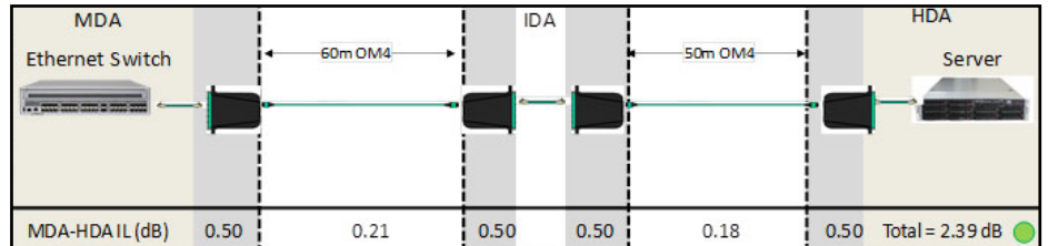
Figure 13. Loss budget calculations for server-to-network link over OM4 fibre
