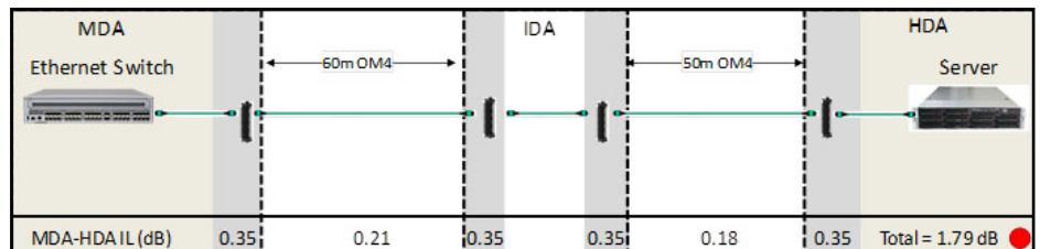
Figure 15. Loss budget calculations for server-to-network link over OM4 fibre—40G upgrade
