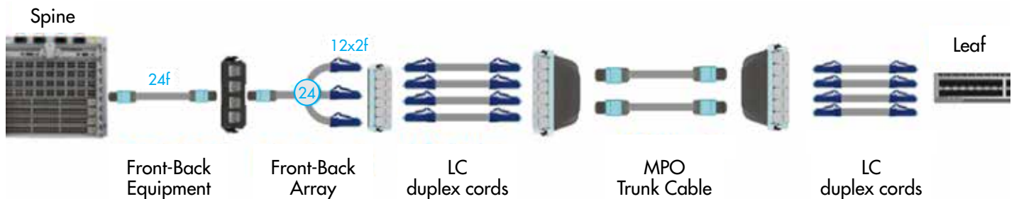
Figure 9. Server-to-leaf connectivity with InstaPATCH 360
