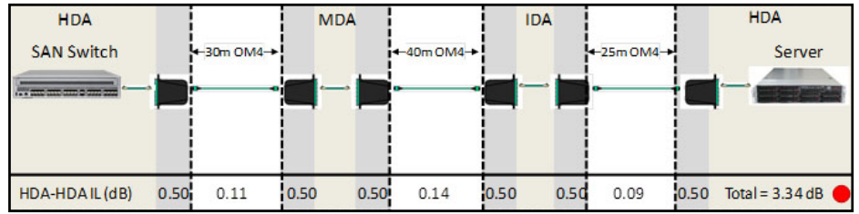
Figure 12. Loss budget calculations for server-to-SAN link over OM4 fibre
