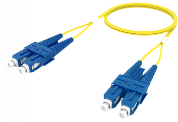
Fiber Optic Patch Cord, Duplex, Singlemode, SC/UPC to SC/UPC, yellow, 20 m
