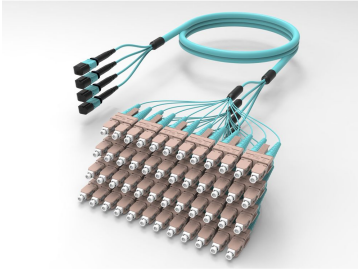
OM3 MPO (Unpinned) to SC/UPC, InstaPATCH® 360 Ruggedized Fanout Cable, 48-Fiber, Plenum
