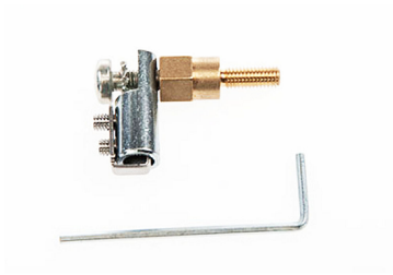
FIST® Universal cable termination kit, central strength member bracket, 6 pcs
