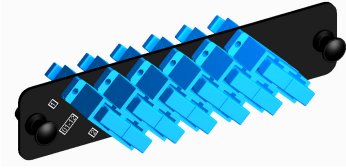
1000-Type Adapter Pack with 6 SC duplex SM adapters, blue
