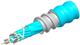
OptiSPEED® Plenum MPO Trunk Cable, interlocking aluminum armored with plenum jacket, 12 fiber
