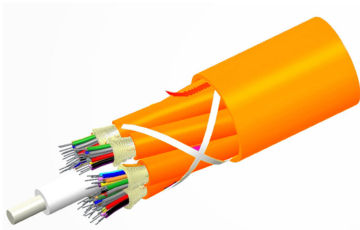
LazrSPEED® Plenum Distribution Cable, 144 fiber multi-unit with 12 fiber subunits
