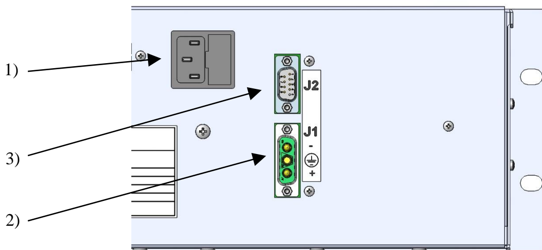
Fig. 5 - Electrical connections
