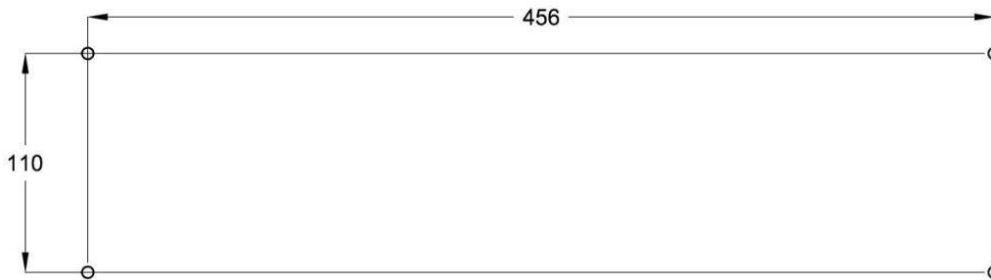
Fig. 3 - Screw hole patterns
