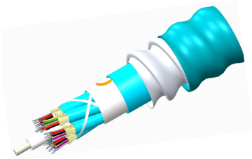
TeraSPEED® Riser Distribution Cable, interlocking aluminum armored with riser jacket, 24 fiber multi-unit with 6 fiber subunits
